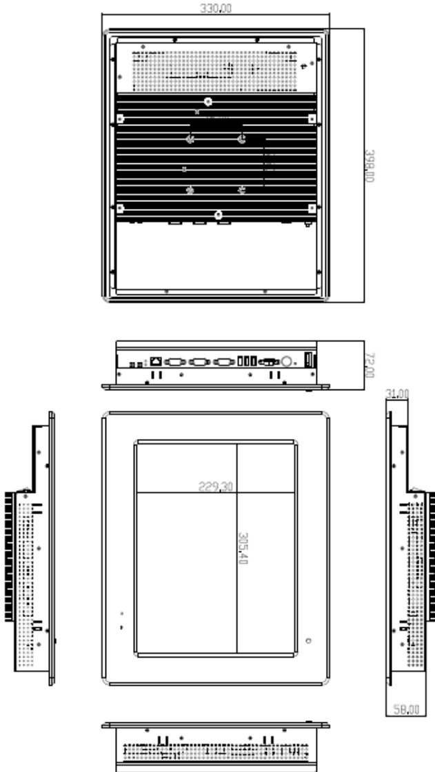
WLP-7920-15H Outline Drawing (Panel Mount)
