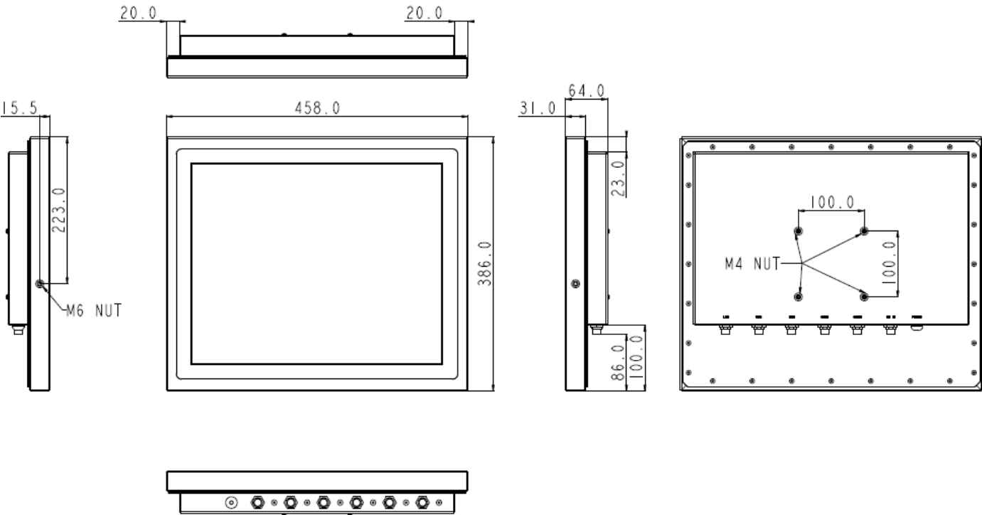
WTP-9A66-19 Outline Drawing
